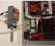
PLC Control system
