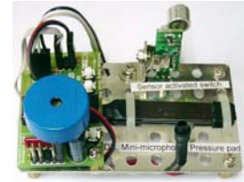
Demo 12 Sensor Activated Switch (Ldr, Mini-microphone, Pressure-pad switch)
