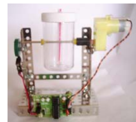
G-GE-FishFeed Fish Feeder Model
