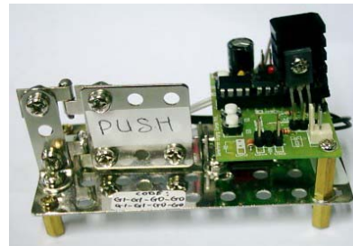
Demo 8 Security Door (Solenoid)
