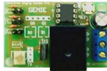
G-GE-2KR Genie Relay
