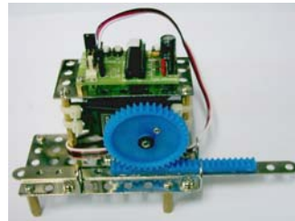
Demo 7 Servo Motor Control (actuator)
